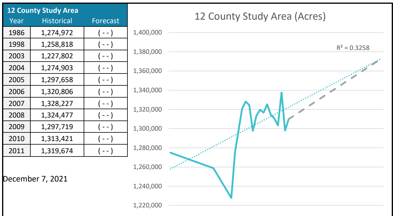
FIGURE 4: FOREST REGRESSION ANALYSIS FOR 12 COUNTY STUDY AREA
